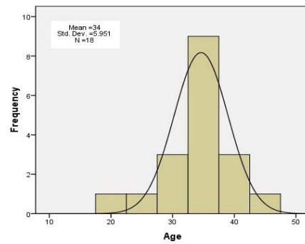
Figure 2 : Frequency Distribution
