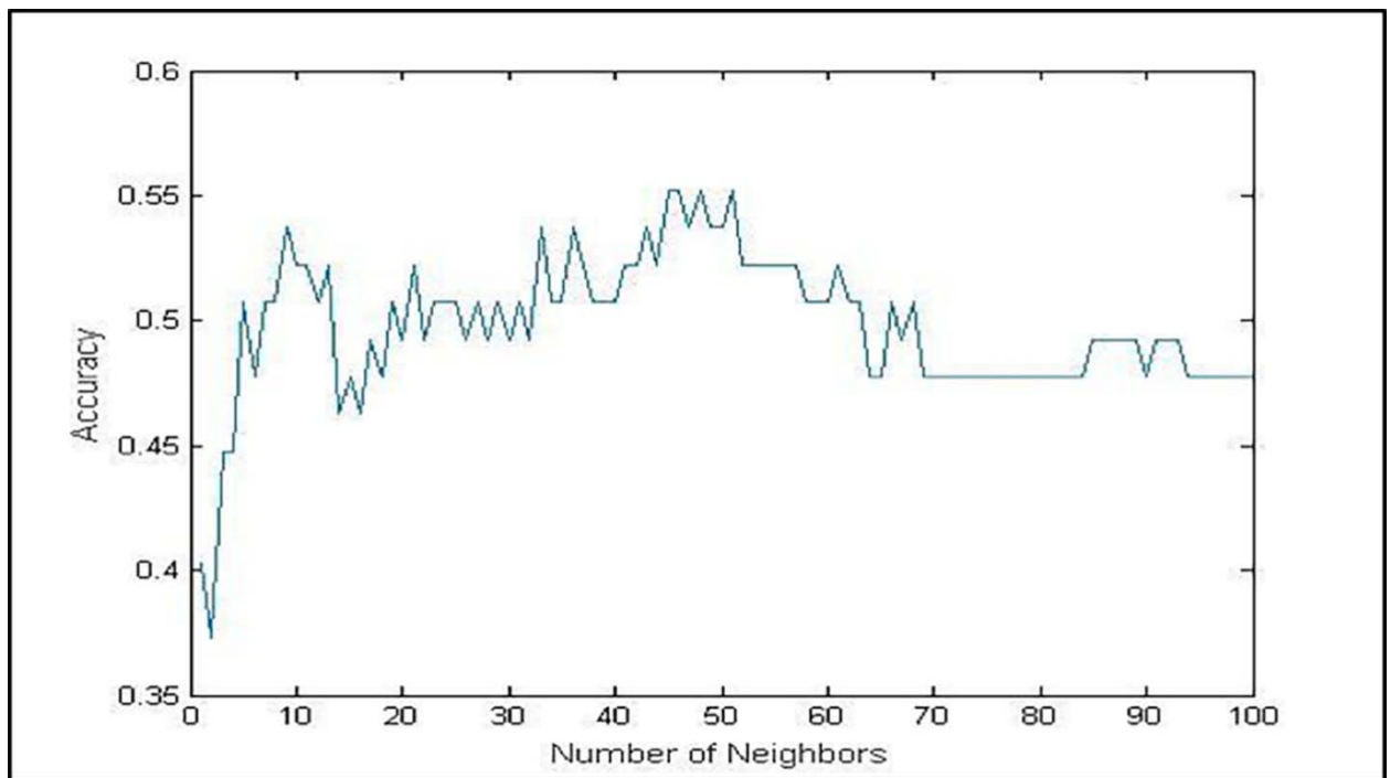
Fig. 4: Accuracy model of UCI dataset
