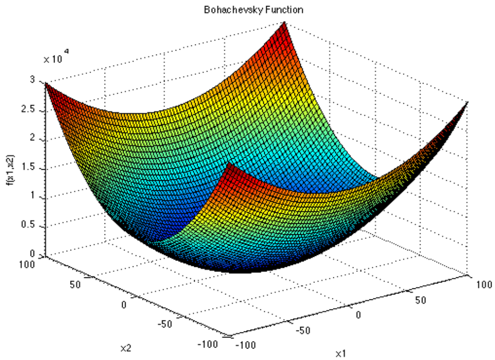
Figure 4: Bohachevsky Function
