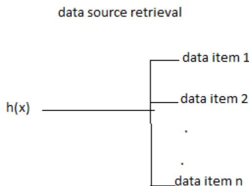
Figure 28: Blackboard System
