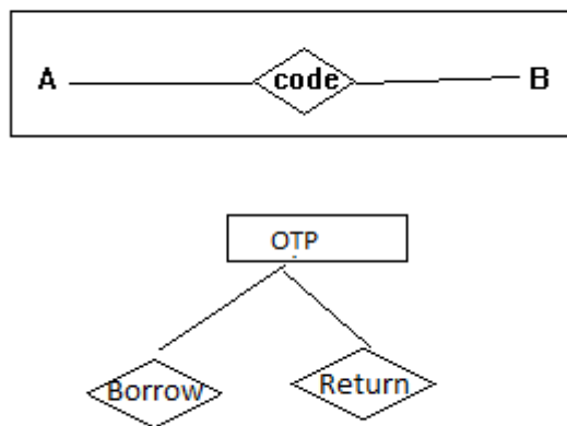
Figure 11: Blockchain
