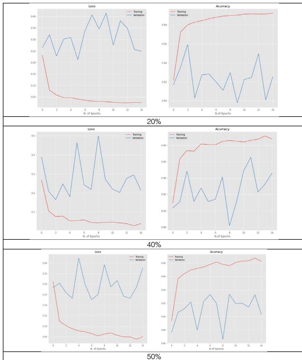
Figure 5: The relationship between accuracy and loss with the number of epochs for the image dataset for the Inception V3 model with 20%, 40%, and 50% dropout values.
