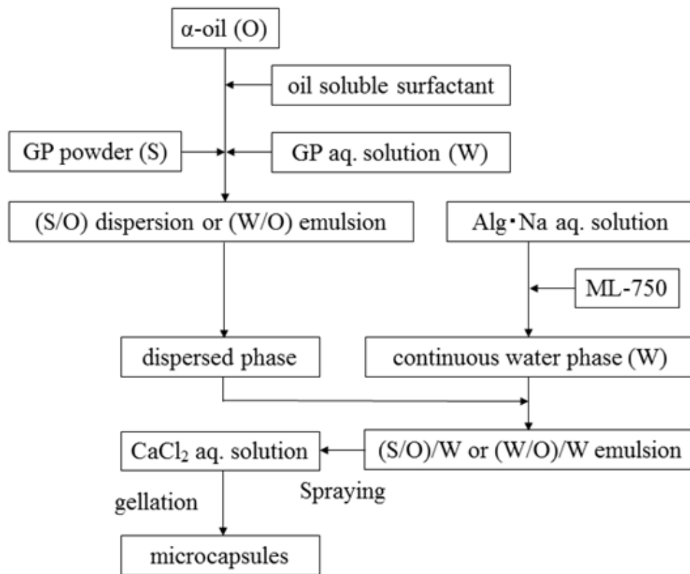
Figure 1 : Flow chart for preparing microcapsules
