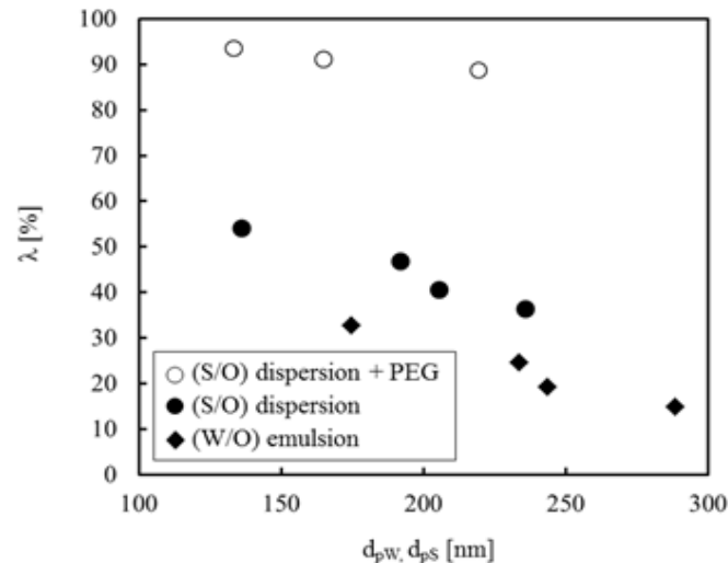
Figure 13 : Dependence of microcapsulation efficiency on inner water droplet diameter and particle diameter
