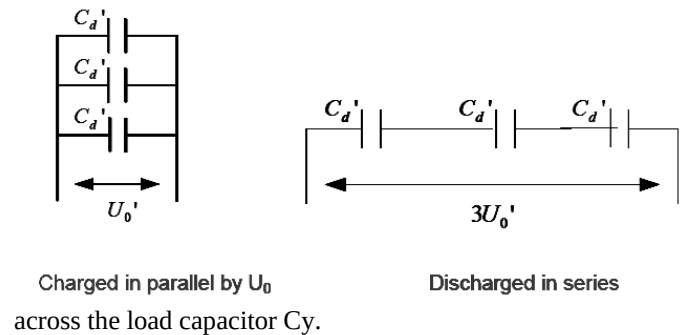
Fig 2: Capacitor orientation for charging/discharging phase
