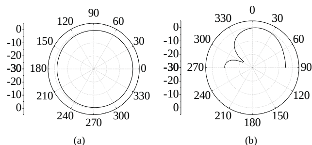
Fig.13 : Radiation pattern (normalized) (a) Total gain in E-plane and (b) total gain in H-plane of IFDL antenna at 5.5 GHz.
