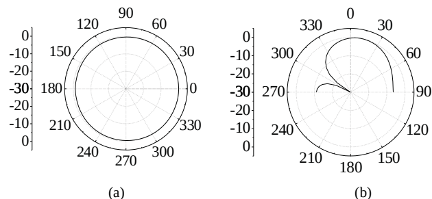
Fig.12 : Radiation pattern (normalized) (a) Total gain in E-plane and (b) total gain in H-plane of IFDL antenna at 5.2 GHz.
