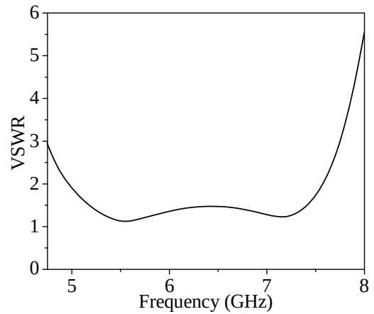
Fig. 7: VSWR variation of IFDL antenna with frequency.
