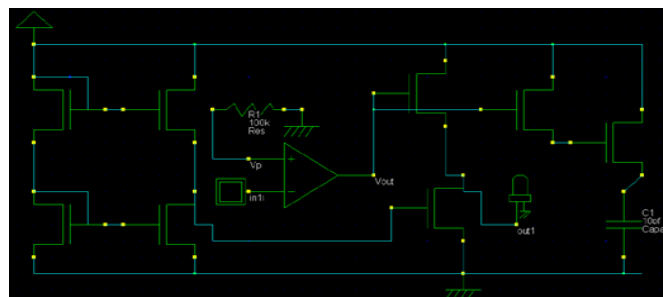
Circuit Diagram of (Fig.) Buffer Amplifier.
