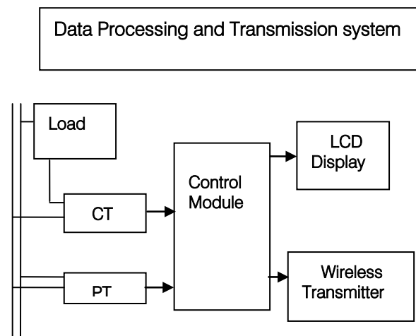
Fig. 2 : Block diagram of the energy meter system showing the subscriber's end.
