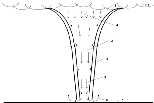
Figure 4: Sketch of tornado. Notations: 1 – charged clouds; 2 – body of tornado; 3 – rotated wall of tornado; 4 – electric intensity; 5 – electron (ion) wind; 6 – exit of electron (discharged) wind; 7 – ground
