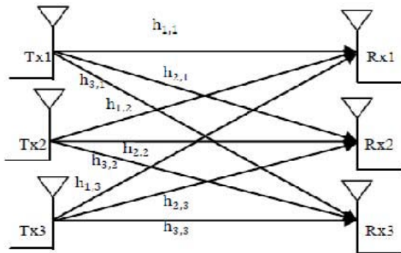
Fig. 3: 3 transmit 3 receive (3 x 3) MIMO channel
