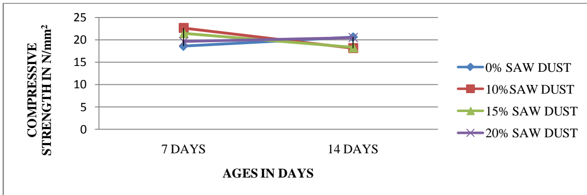
Figure 2 : Variation of Compressive strength with age and percentage of saw dust
