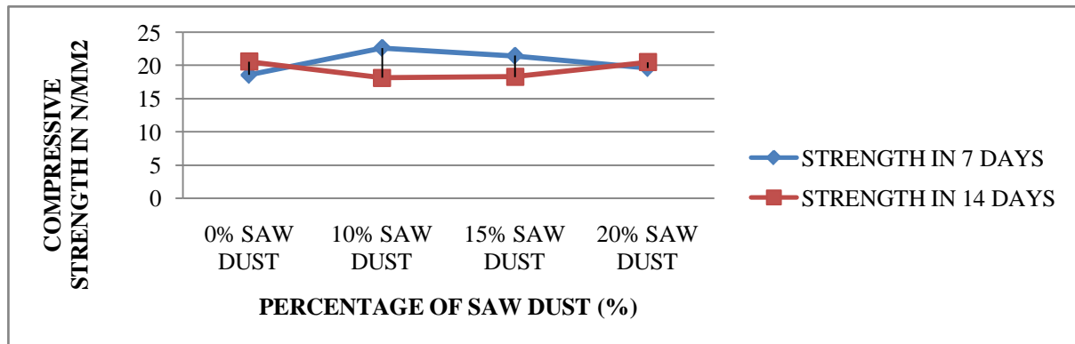
Figure 3 : Percentage of saw dust v/s Compressive strength
