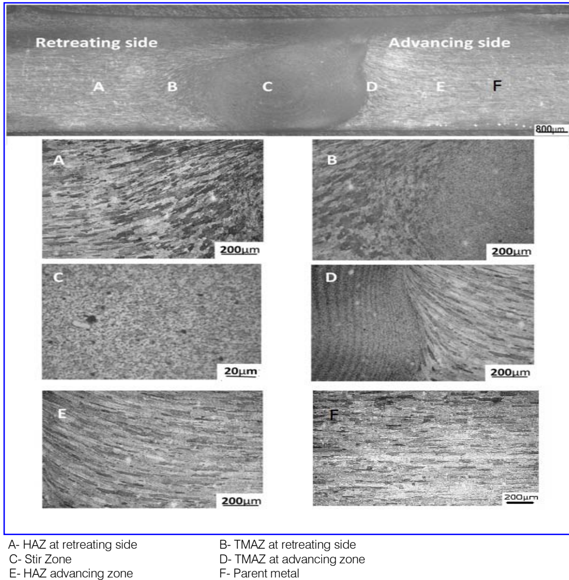
Fig. 6 : Microstructures at different zones of a friction stir welded joint with 3^\circ tool tilt angle
