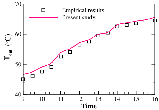
Figure 2: Comparison of the present results with the empirical results of Khorasanizadeh et al. [2], in term of outlet fluid temperature
