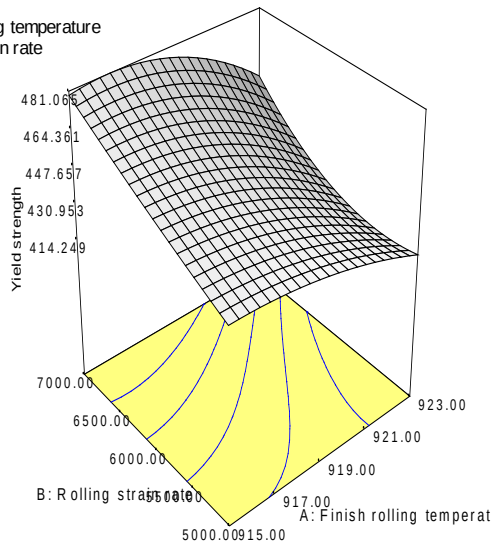
Fig. iii: Surface plot for yield strength
