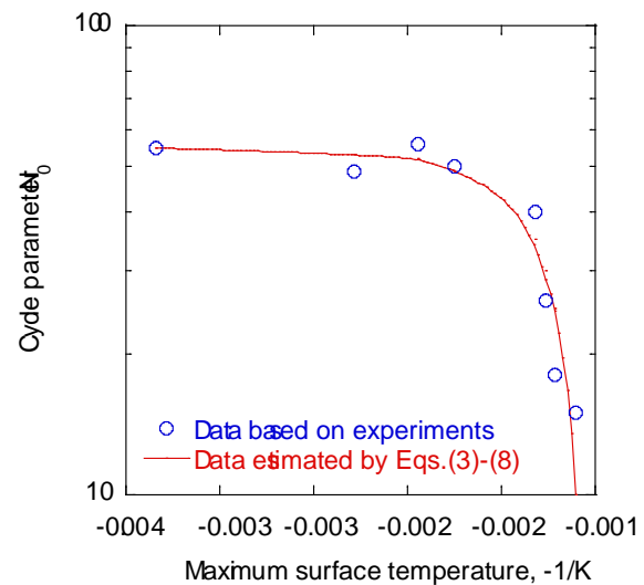
Figure 13: Relationship between cycle parameter and the maximum surface temperature just before processing starts
