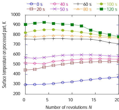
Figure 7: Change in maximum surface temperature on the processed part with the increase in number of revolutions in each heating time ( \theta = 3^\circ , \sigma_c / \sigma_y = 0.97 )
