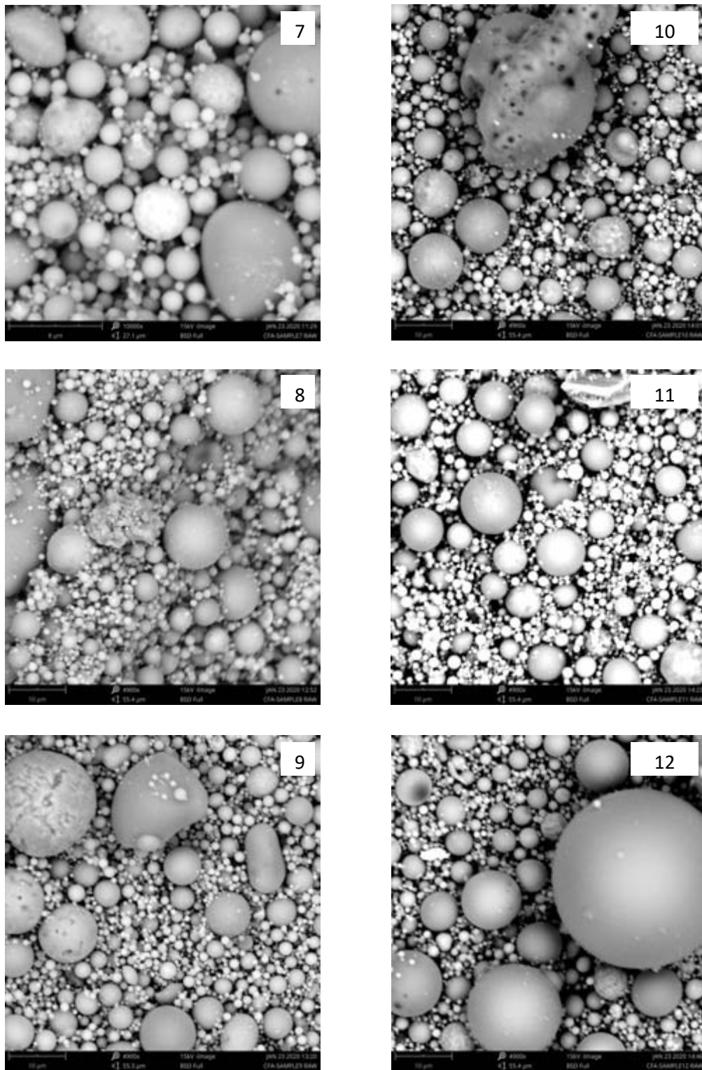
Figure 2: SEM Photographs of the different coal fly ash samples. (Class-F fly ashes: 1-5; Class-C fly ashes: 6-12)
