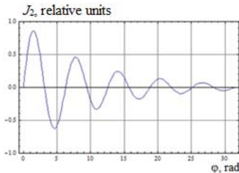
Fig. 6: Functional dependence of the current in the load normalized to the maximum
