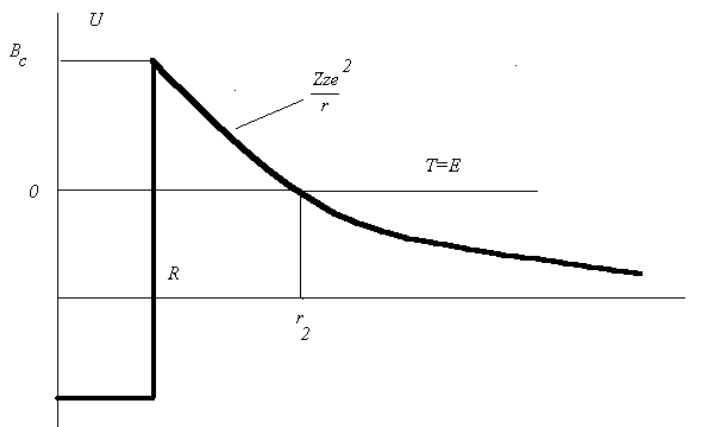
Fig. 1 : Potential corresponding to nuclear fusion
