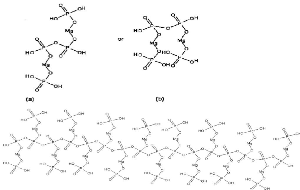
Figure 5 : Polymerization steps showing metal tetraphosphate dimer of less-stable (b) and more-stable (a) forms, plus the stable form of a multidimensional polymer (brickwall-like structure). Magnesium is shown as an example of a metal [12]
