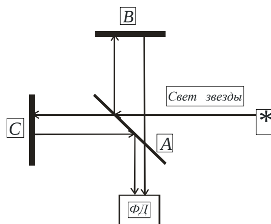
Fig. 1: Schematic of Michelson interferometer
