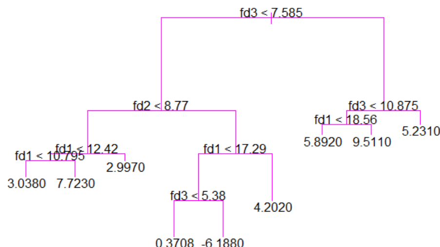
Figure 2: Unpruned Regression tree with 9 terminal nodes (leaves) and 8 internal nodes. This regression tree model shows that fd_3 which is the measure of stock market liquidity is the most important regressor in the model since it minimizes the RSS in equation 1.0. Splitting was done in such a way that at each step, one of the regressor is selected. At a given internal node, the left-hand branch is represented by X_j < q_k resulting from the split and X_j > q_k indicates the right hand branch. At the top of the tree, the split resulted in two branches in which the left hand branch corresponds to fd_3 < 7.585 per cent and the right hand branch corresponds to fd_3 \geq 7.585 per cent. Splitting ensures simplicity and ease of interpretability of the regression tree model. Source: Computations using R language.
