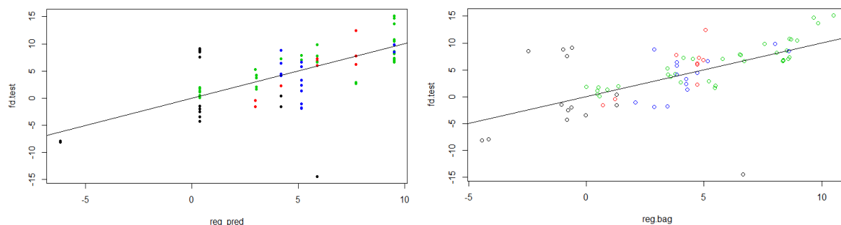
Figure 4: Left panel: The scatter plot on the residuals of the optimally-pruned regression tree using the test dataset. Right Panel: The scatter plot on the residuals of the aggregated bootstrapping on G = 200 regression trees using the test dataset (i.e. Bagging procedure). The straight line through the dotted points is the trend line. Source: Computation using R language
