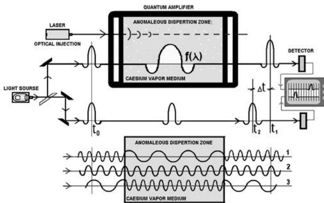
Fig. 5: Experiments of L. Wang - superluminal light propagation
