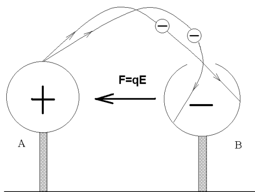
Fig. 8: Work for transferring the charge depends on the mode of transferring and on the path
