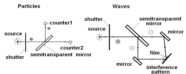
Fig. 1: Experiments with individual photons on semitransparent mirror
