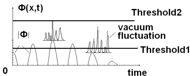
Fig. 4: Quantum measurements
