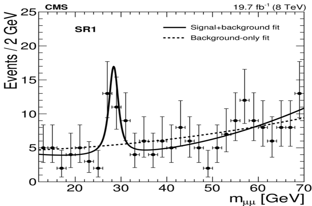
Fig. 6: Peak of energy at 28GeV
