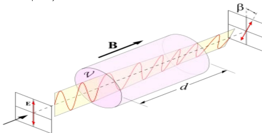
Fig. 1: Rotation of plane of polarization of light within a medium due to external magnetic field
