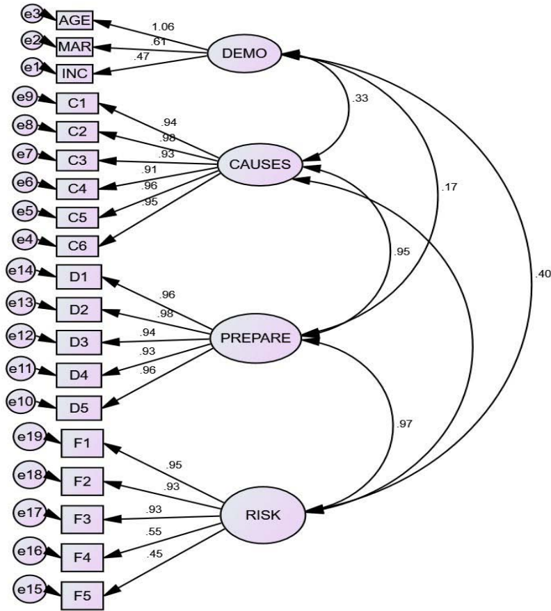
Figure 2: Confirmatory Factor Analysis (CFA)
