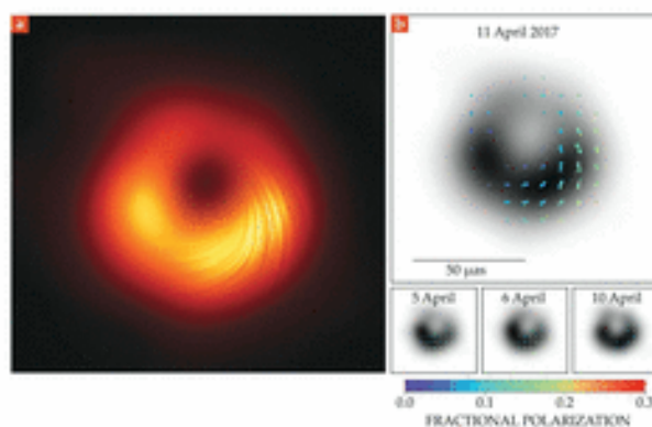
Fig. 1: Photo of the Black Hole of the elliptical galaxy Messier 87 in polarized light
