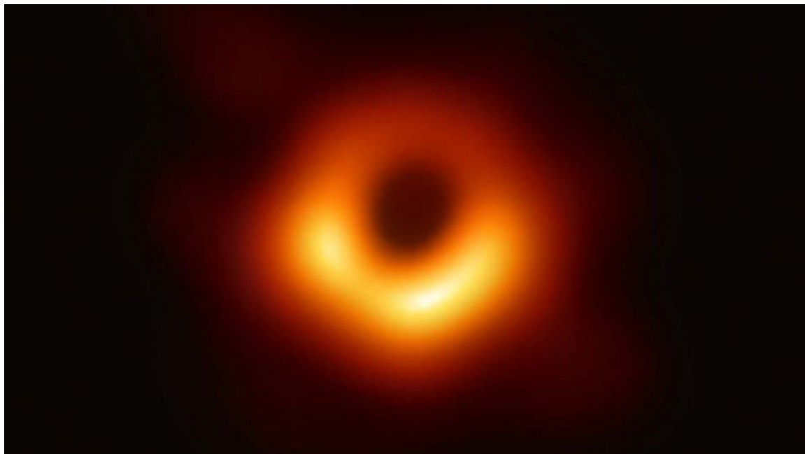
Fig. 3: First EHT photo of the Black Hole of the elliptical galaxy Messier 87
