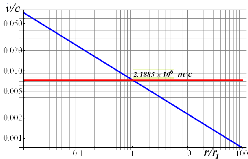
Fig. 1: The dependence of the relative (reduced to the speed of light) velocity of the steady motion of an electron in the orbit of a hydrogen atom on the relative radius of the electron orbit, reduced to its experimental radius (blue line): e = -1.60 \cdot 10^{-19} \text{ C} , m = 9.11 \cdot 10^{-31} \text{ kg} , \epsilon_0 \approx 8.85 \cdot 10^{-12} \text{ m}^{-3} \text{ kg}^{-1} \text{ s}^4 \text{ A}^2 , r_1 = 53 \cdot 10^{-12} \text{ m}
