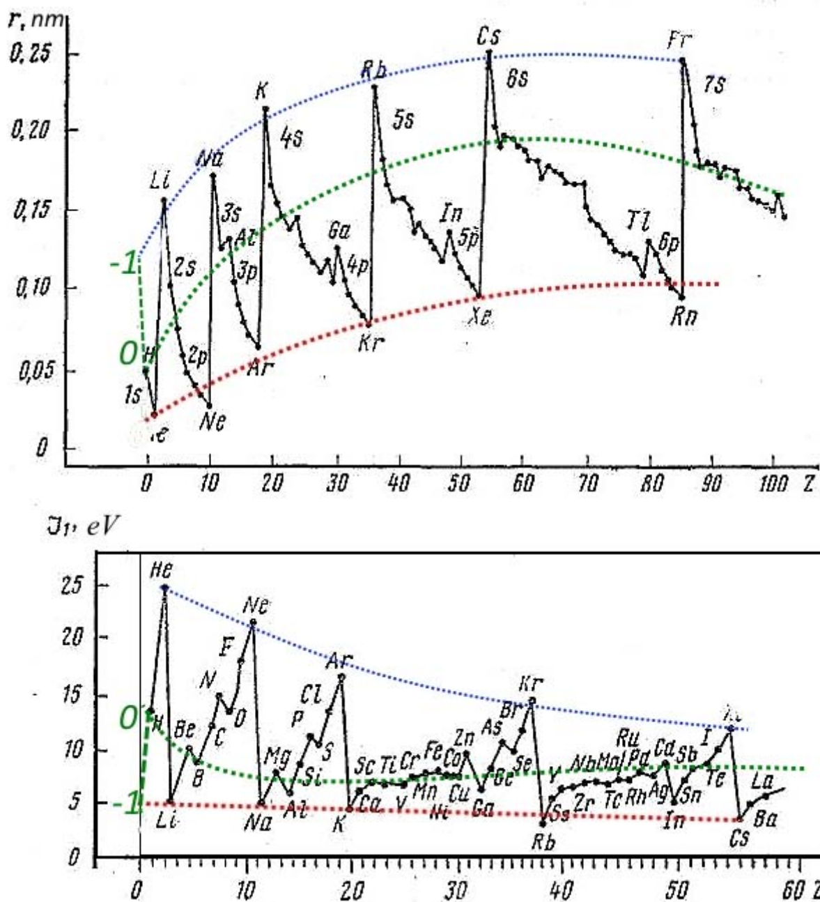
Fig. 4: Dependence of the radius of the outer electron shell and its First Ionization Potential on the atomic number (Zero denotes the “zero” element used in the construction of the periodic table by Mendeleev, and minus one is an additional conditional element with minus one electron)
