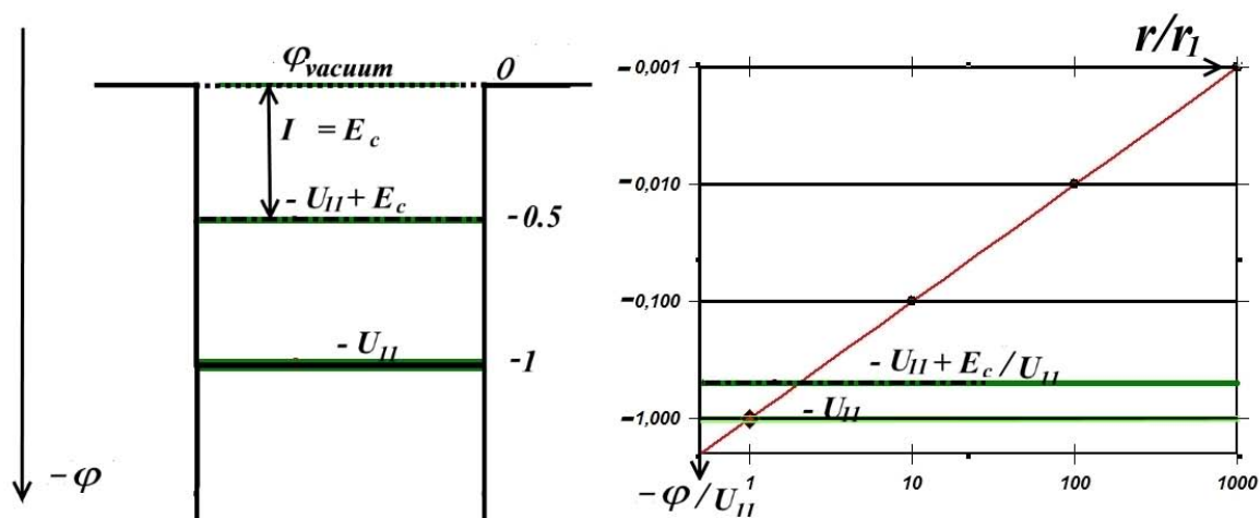
Fig. 2: Electron energy level diagram on a linear scale (left) and on a logarithmic scale (right) the edge of the potential Coulomb well (red line) with exponentially decreasing equipotentials with the electron energy level superimposed on them (green line).
