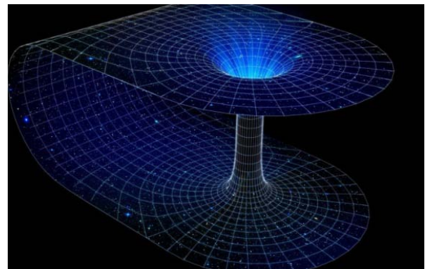
Figure 1: Wormhole (walkable)
