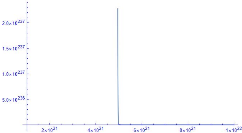
Fig. 4: The Energy Density [ J / m 3 ] of the Dark Matter as a function of the Radius R = max 10 22 [m]
