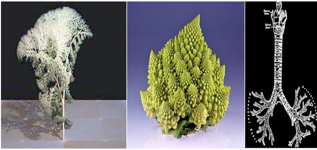
Figure 5. Fractal tree (left), kale (center), trachea (right).
