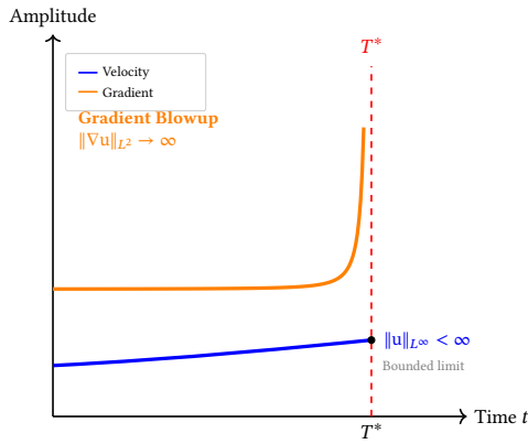
Figure 1. Loss of regularity at T^* . The derivative (orange) diverges as it approaches the singular time, while the velocity amplitude (blue) remains bounded at a finite value.
